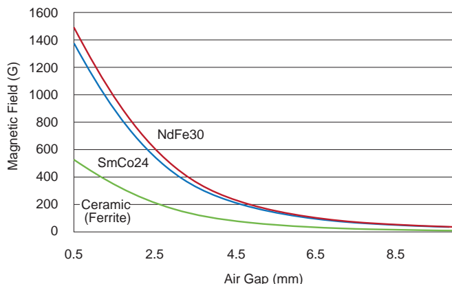
Figure 32: Magnetic Field versus Air Gap for a magnet 6 mm in diameter and 2.5 mm thick.
