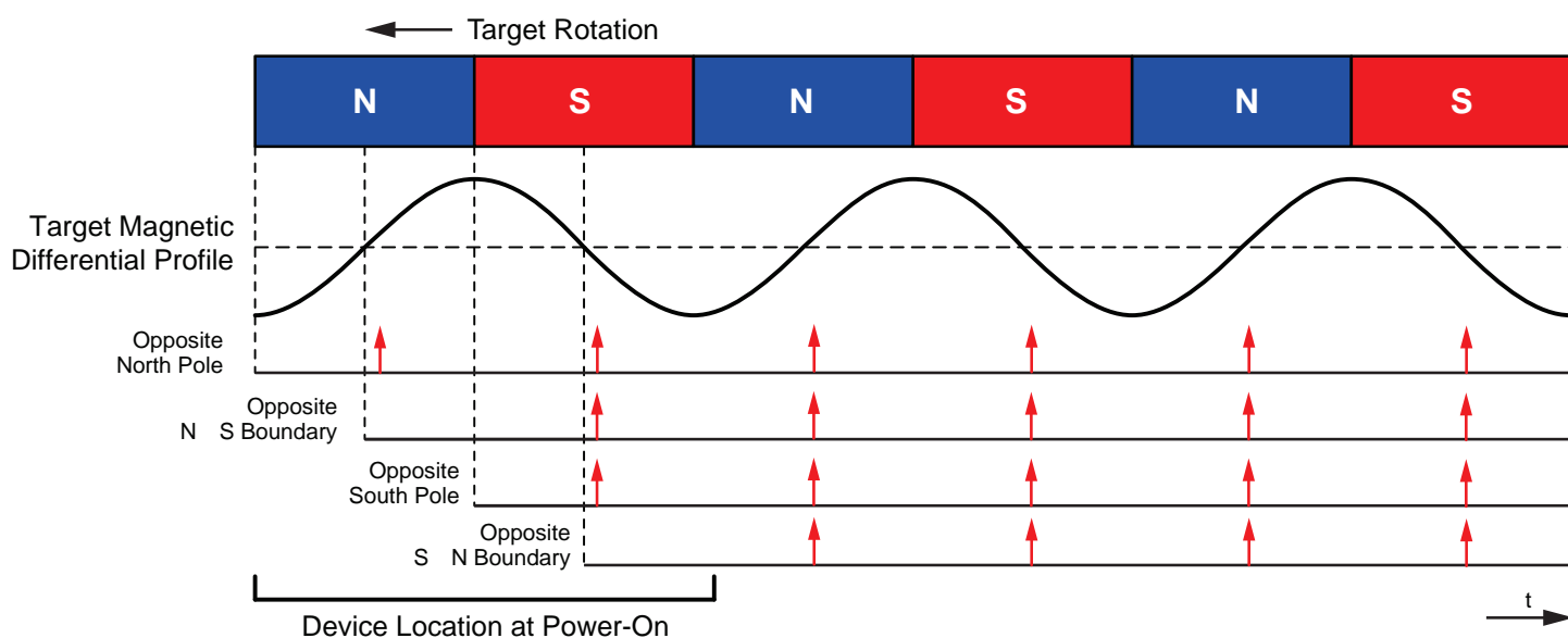
Figure 11: Calibration Behavior (-xBx Variant)
