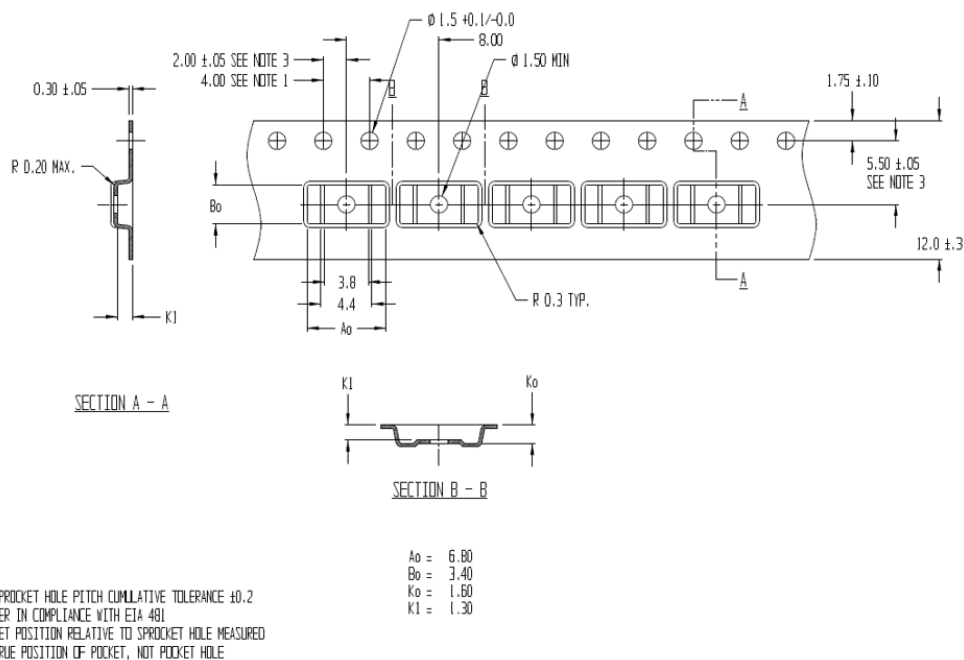
Figure 41: Tape and Pocket Drawing for TSSOP-8 Package
