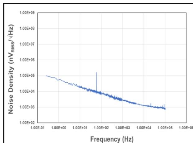
Figure 25: Noise Density vs. Frequency
