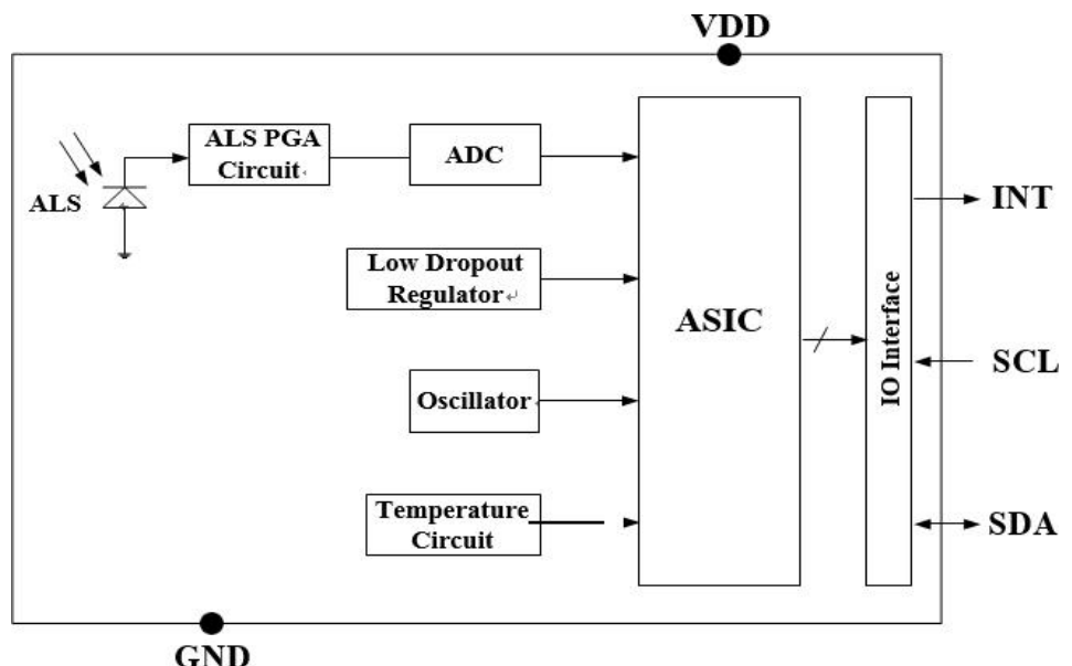
Fig. 1 Block Diagram
