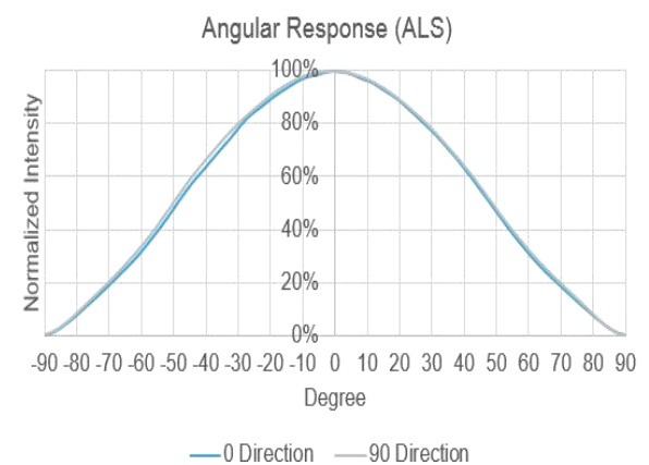
Fig. 2 Angular Response
