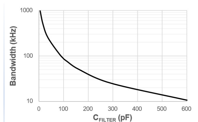
Figure 16: Bandwidth vs. C_{FILTER}
